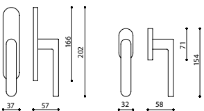
C200R - fixed window slider
